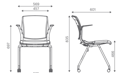
4 Legged Stacking Castor 4-M8PL-0000-M043-M364-A
