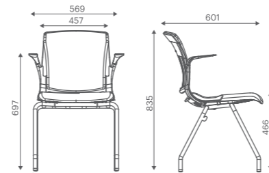
4 Legged Stacking Glide 4-M8PL-0000-M043-M354-A
