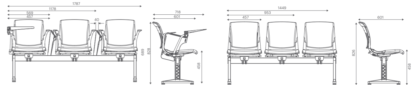
4 Legged With Tray 4-M8PL-0000-M043-M374-A
