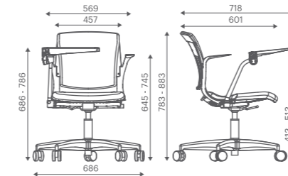
Team Base Height Adjustable 4-M8PL-M023-M054-T123-A
